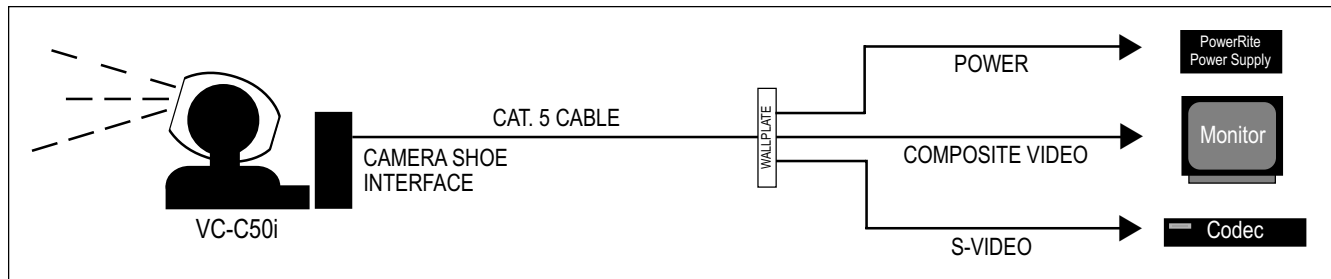
Figure 1 – EZCamera cable system with a quick-connect single gang wallplate/quick-connect box.
